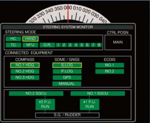
(Monitor Screen) Integrated Steering system monitoring information can be displayed. Steering Mode, Rudder condition, and the condition of interfaced sensors can be understood at a glance.
